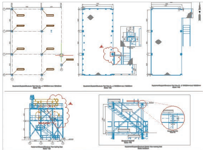
A structural layout drawing
